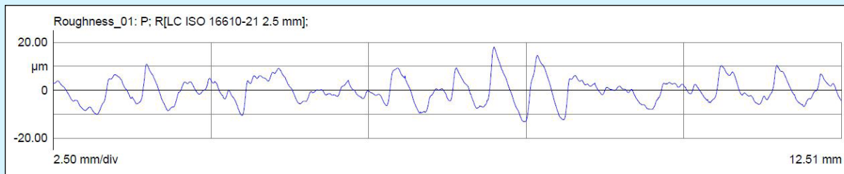
Data from surface roughness testing on one side of a legacy stereolithography part
